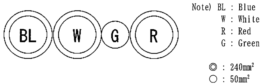
Fig.2 Core identification
