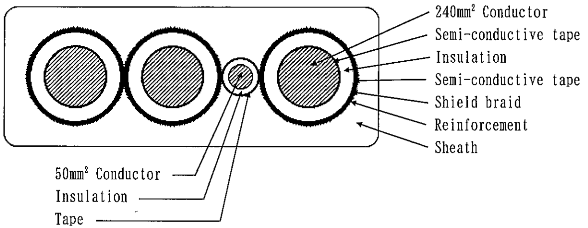
Fig.1 Cable cross section
